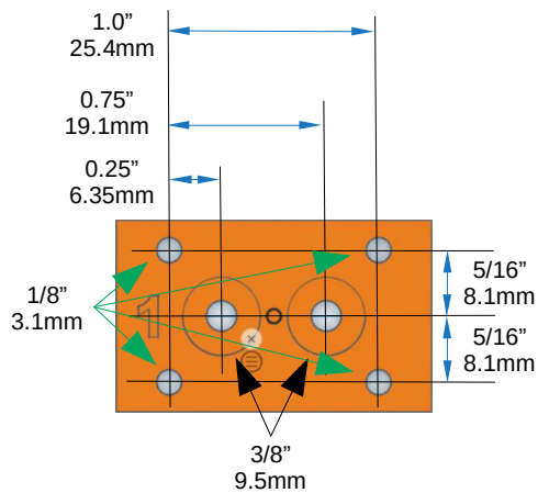
DF2P-00104 2 Post Deployment Feedthru
