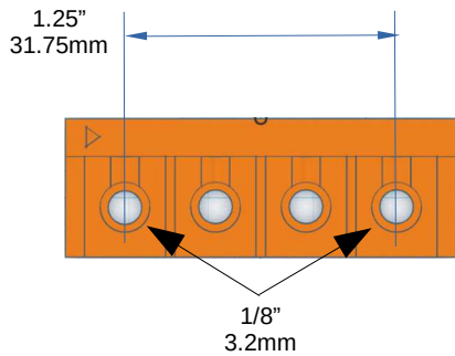
CB4TM-00106 4 Terminal Through Mount Connector Block
