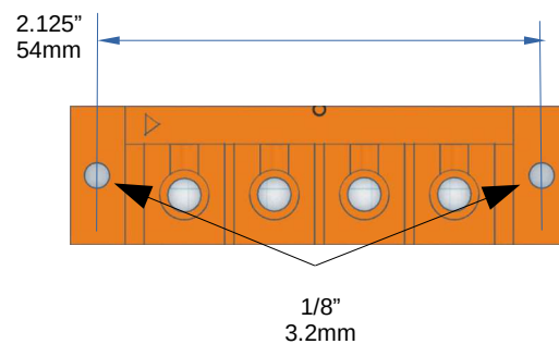
CB4EM-00107 4 Terminal Tab Mount Connector Block
