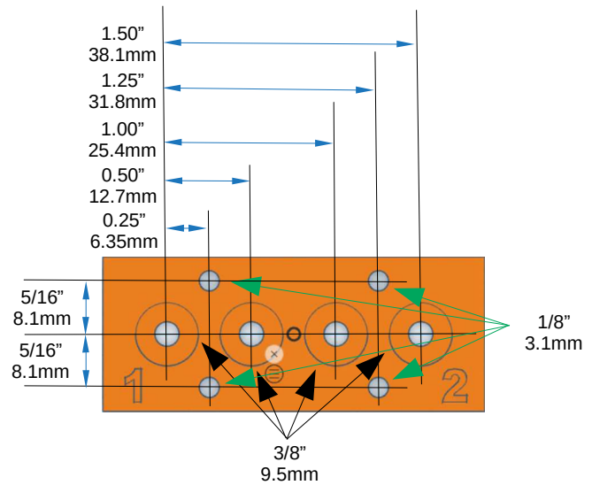
DF4P-00105 4 Post Deployment Feedthru
