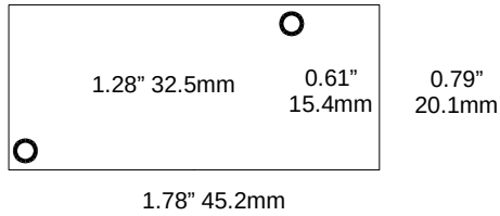
Raven3
