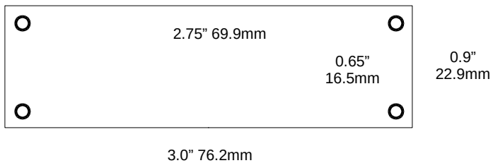
miniAlt/WD+
